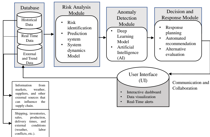
Fig. 1 Proposed IDSS for anomaly detection in the supply chain.
